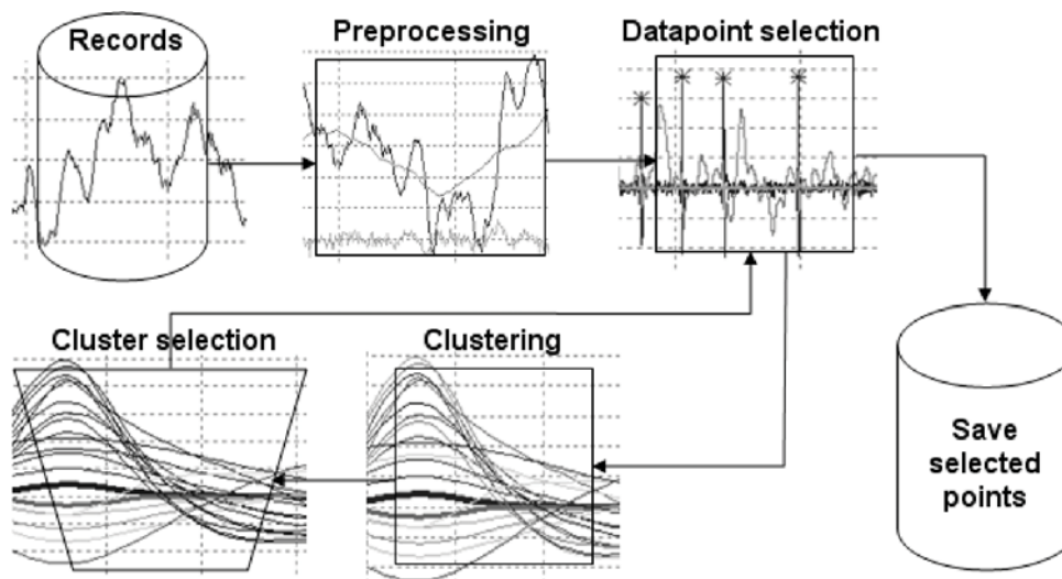
Fig. 1: Algorithm flowchart.
